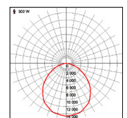
300W-5000K-120°
